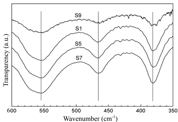
Figure 2. The FTIR spectra of: zeolite A (S9), after introduction of iodine into ZA (S1), sample obtained after heating of S1 at 210 °C for 3 h (S5), and after heating of S1 at 410 °C (S7).
